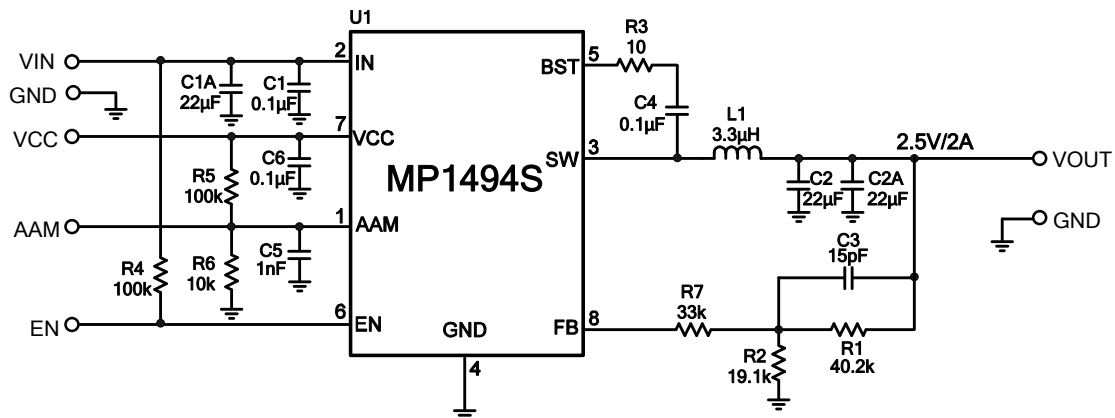
Figure 9: 12V IN , 2.5V/2A Output
