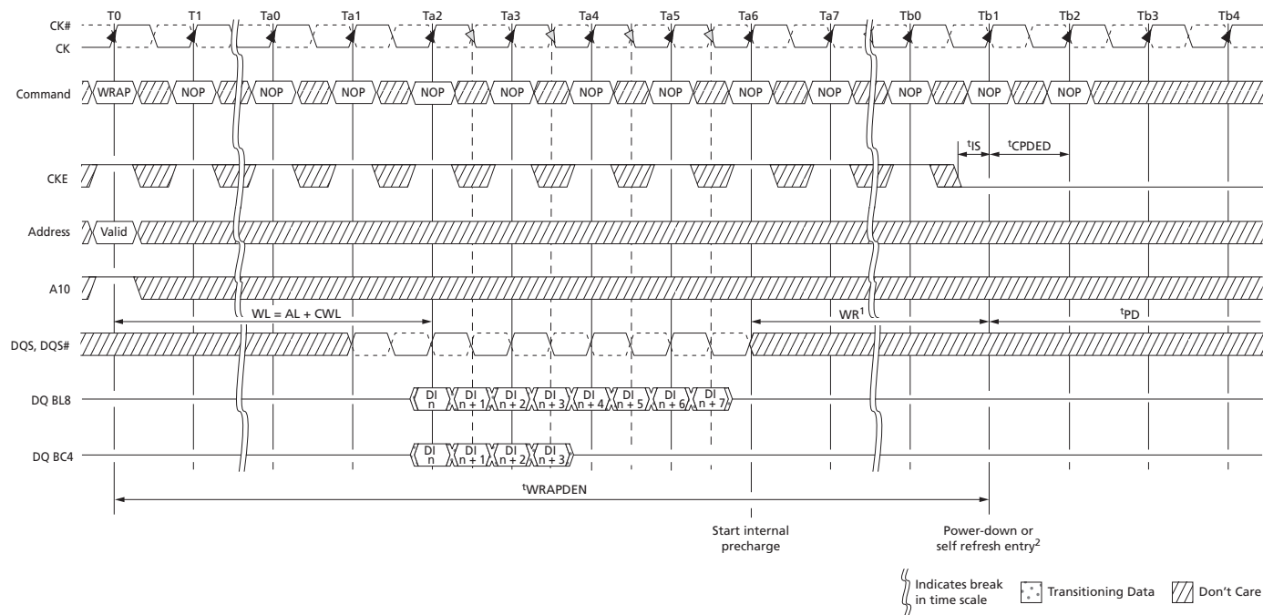
Figure 98: Power-Down Entry After WRITE with Auto Precharge (WRAP)
