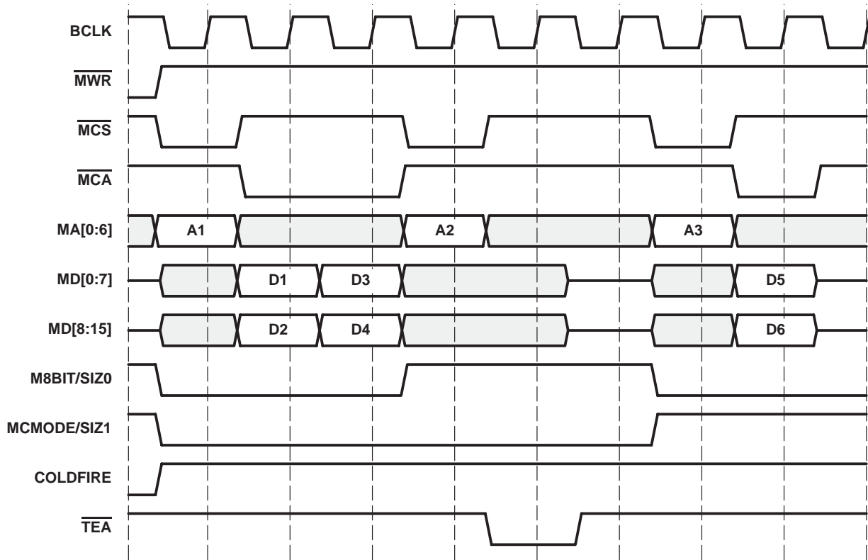
Figure 3–13. ColdFire Read
