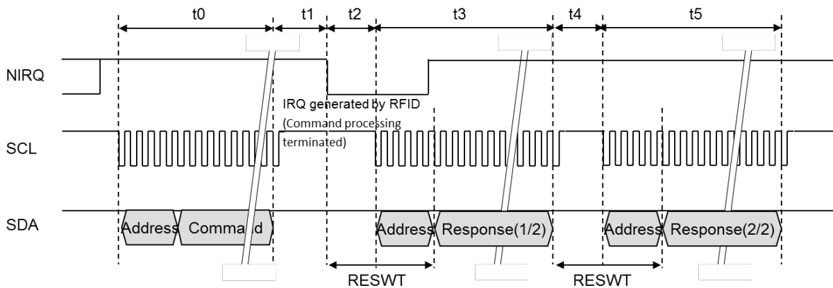
Figure 5-5 Time Chart of Divided Response Access
