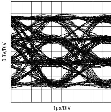
4-Level, 400kbps (200kps) Eye Diagram
