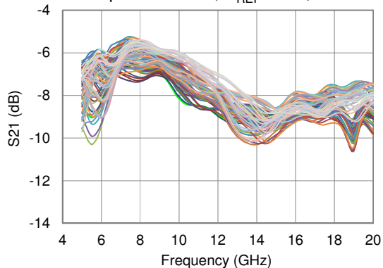
Insertion Loss vs. Frequency All phase states; V_{REF} = 5\text{ V} , 25 °C
