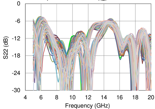
Output Return Loss vs. Frequency All phase states; V_{REF} = 5\text{ V} , 25 °C
