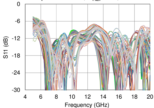
Input Return Loss vs. Frequency All phase states; V_{REF} = 5\text{ V} , 25 °C
