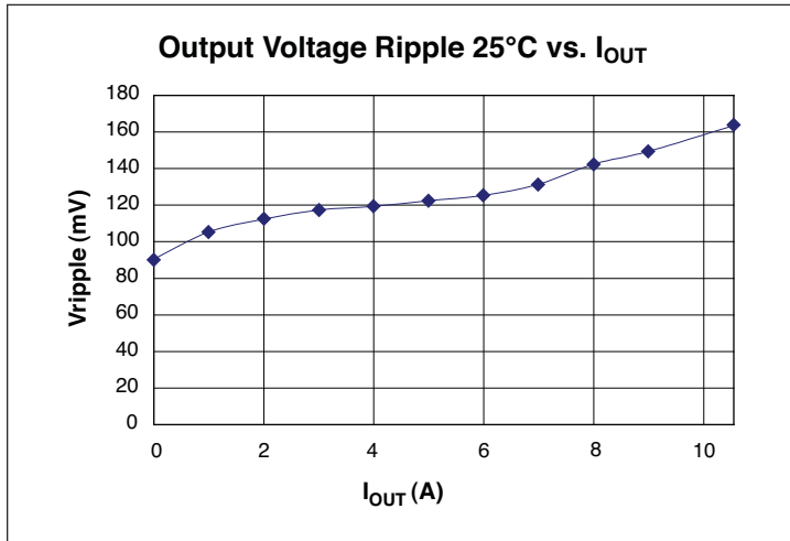
Figure 7 – Ripple vs. I_{OUT} ; 48 Vin, no external capacitance
