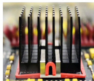
superGRIP™ Assembly
