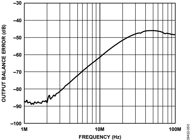
Figure 47. Output Balance Error vs. Frequency
