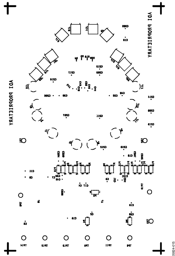
Figure 10. Bottom Silkscreen
