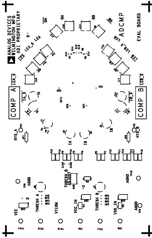
Figure 9. Top Silkscreen
