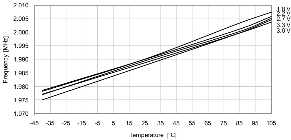
Figure 33-200. 2MHz Internal Oscillator Frequency vs. CALA Calibration Value
