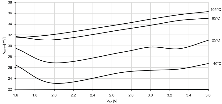
Figure 33-324. Analog Comparator Hysteresis vs. V_{CC} Large hysteresis
