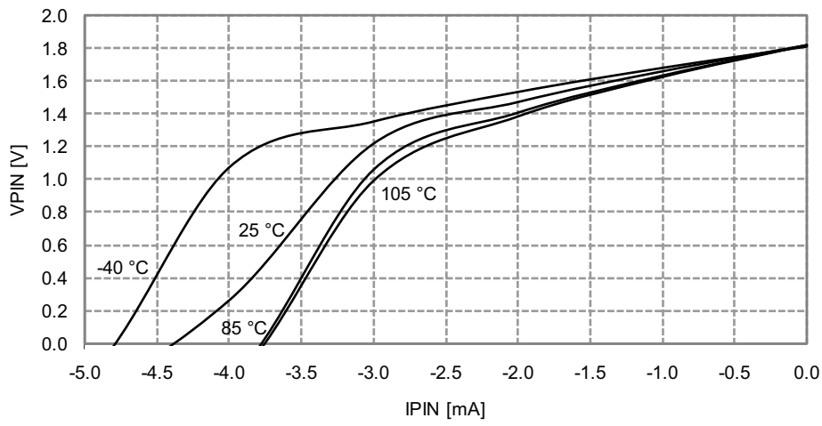
Figure 33-304. I/O Pin Output Voltage vs. Source Current
