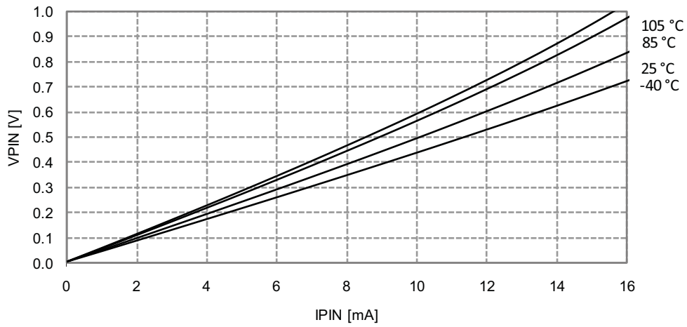
Figure 33-308.I/O Pin Output Voltage vs. Sink Current
