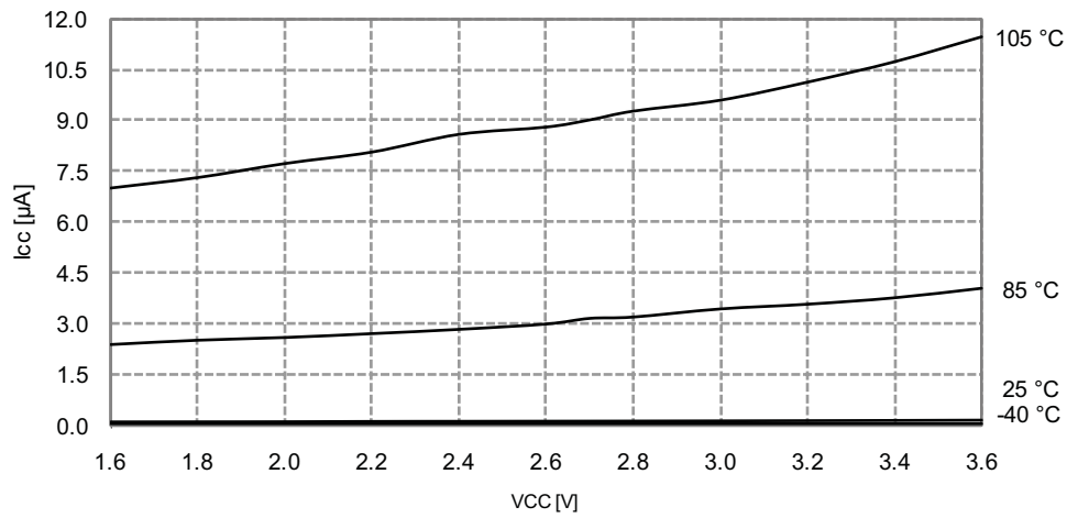
Figure 33-298. Power-down Mode Supply Current vs. V_{CC} Watchdog and sampled BOD enabled
