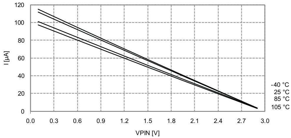
Figure 33-302. I/O Pin Pull-up Resistor Current vs. Input Voltage
