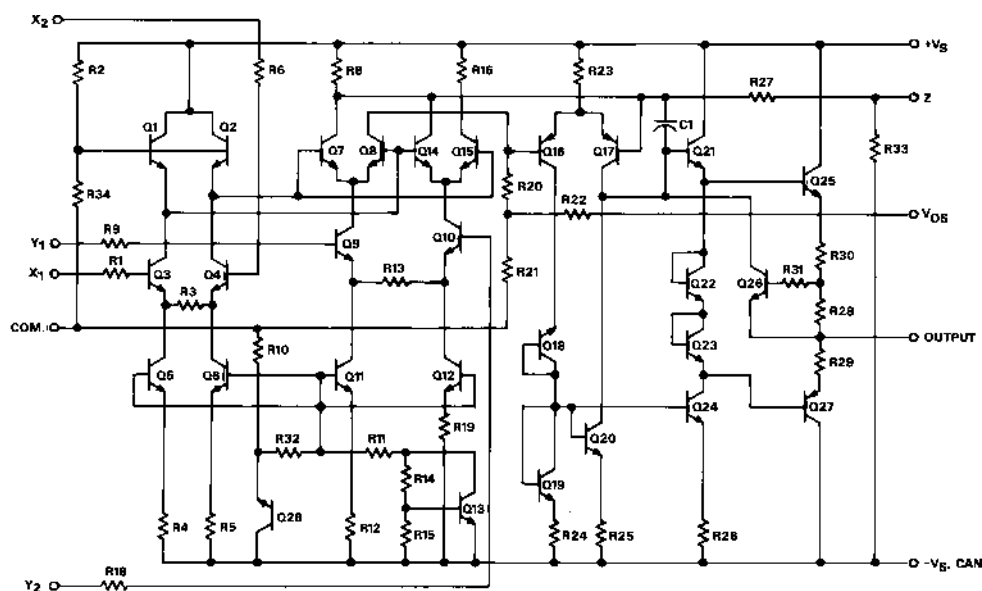
Figure 2. Schematic Diagram
