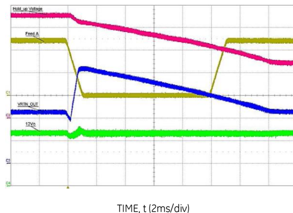
Fig 4: Hold-up Event vs 12.0Vout
