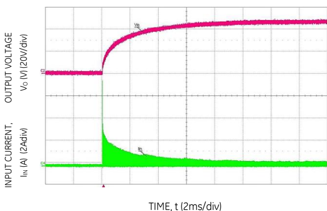
Figure 1. Inrush Current
