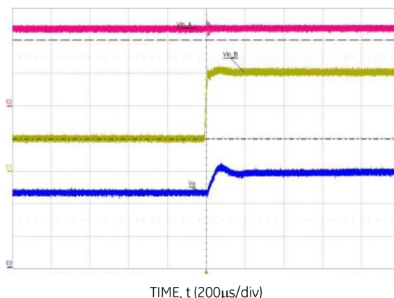
Fig 2: Input Transient on one feed
