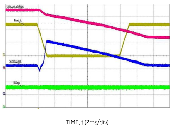
Fig 3: Hold-up Event vs 3.3Vout
