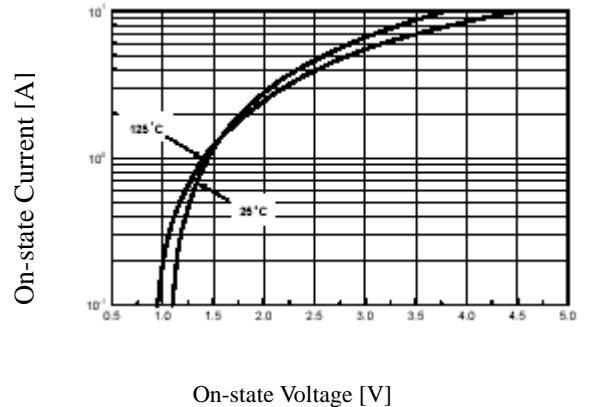
Fig 2. On-State Voltage
