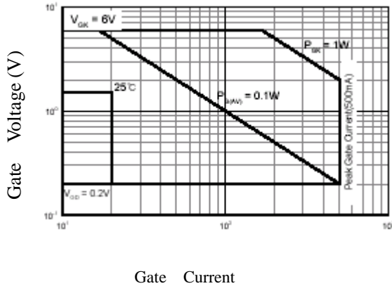
Fig 1. Gate Characteristics
