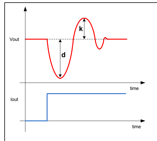
Figure 28 – load step response example and “kick” vs. “droop” definition
