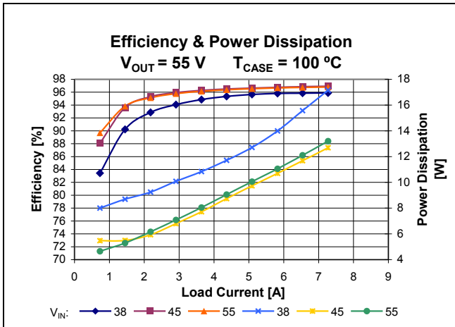
Figure 11 – Total efficiency and power dissipation vs. V_{IN} and I_{OUT} , V_{OUT} = 55 V, T_{CASE} = 100^{\circ}\text{C}
