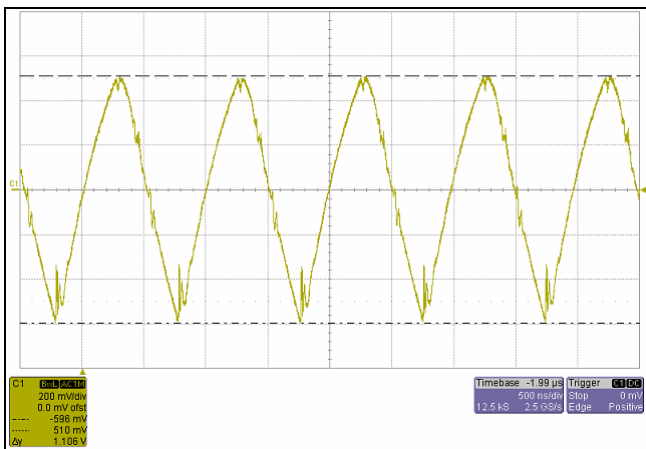
Figure 13 – Typical output voltage ripple waveform, T_{CASE} = 30^{\circ}\text{C} , V_{IN} = 45 V, V_{OUT} = 48 V, I_{OUT} = 8.33 A, no external capacitance.
