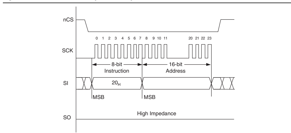
Figure 7-25. SECTOR-ERASE Operation Sequence for Extended Mode
