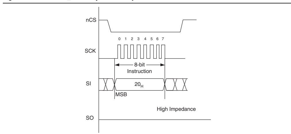
Figure 7-26. SECTOR_ERASE Operation Sequence for Base Mode
