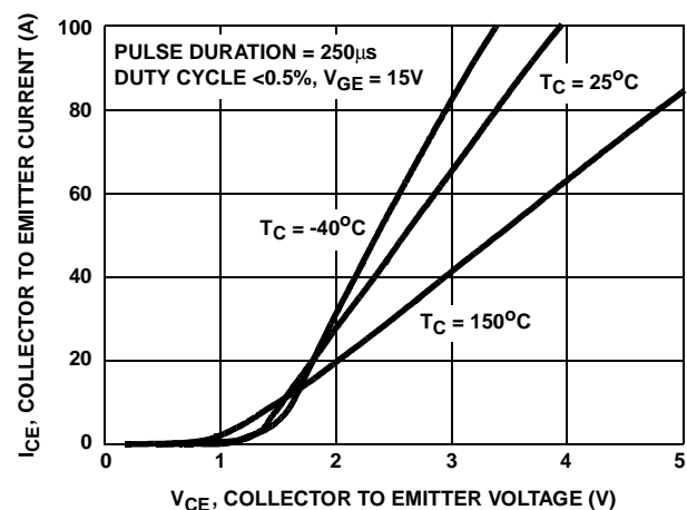
FIGURE 4. COLLECTOR TO EMITTER ON-STATE VOLTAGE
