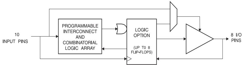
Figure 1-1. Block Diagram
