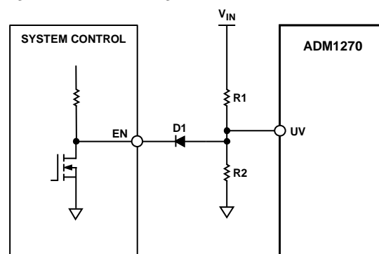
Figure 41. Using the UV Pin as an Enable
