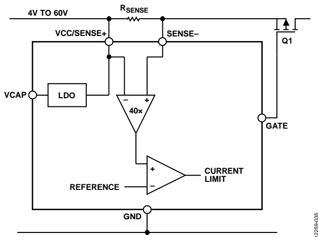
Figure 35. Hot Swap Current Sense Amplifier
