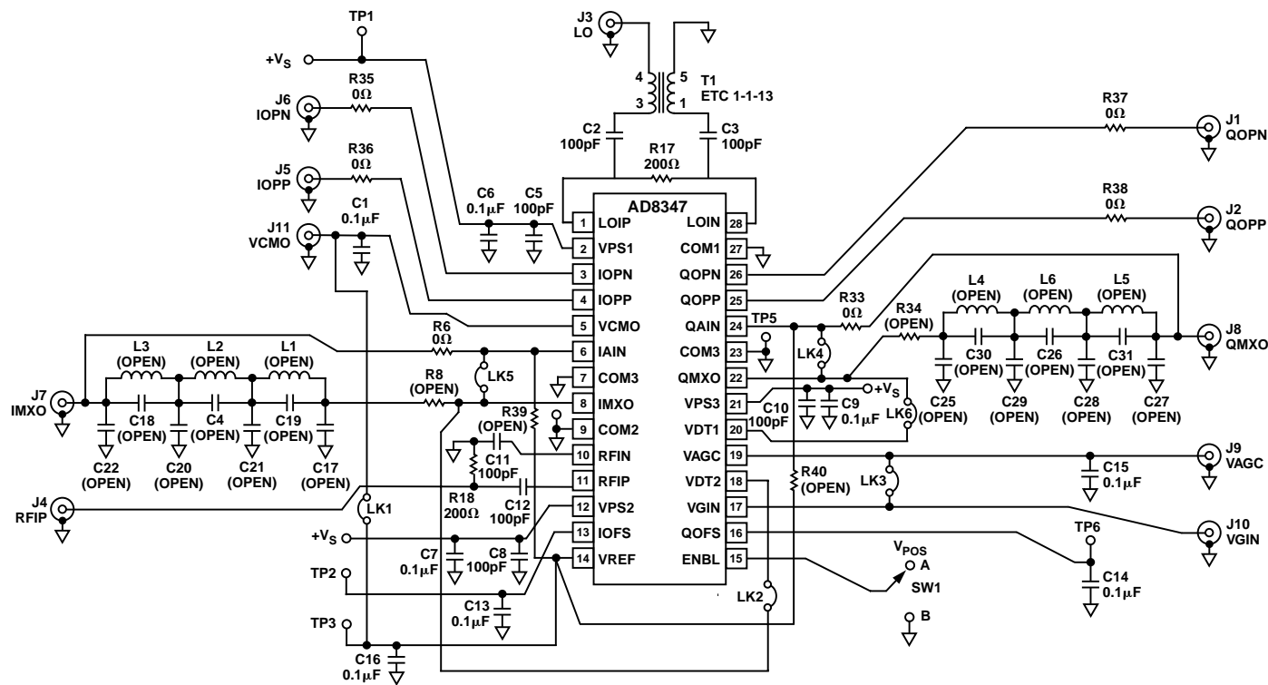
Figure 11. Evaluation Board Schematic
