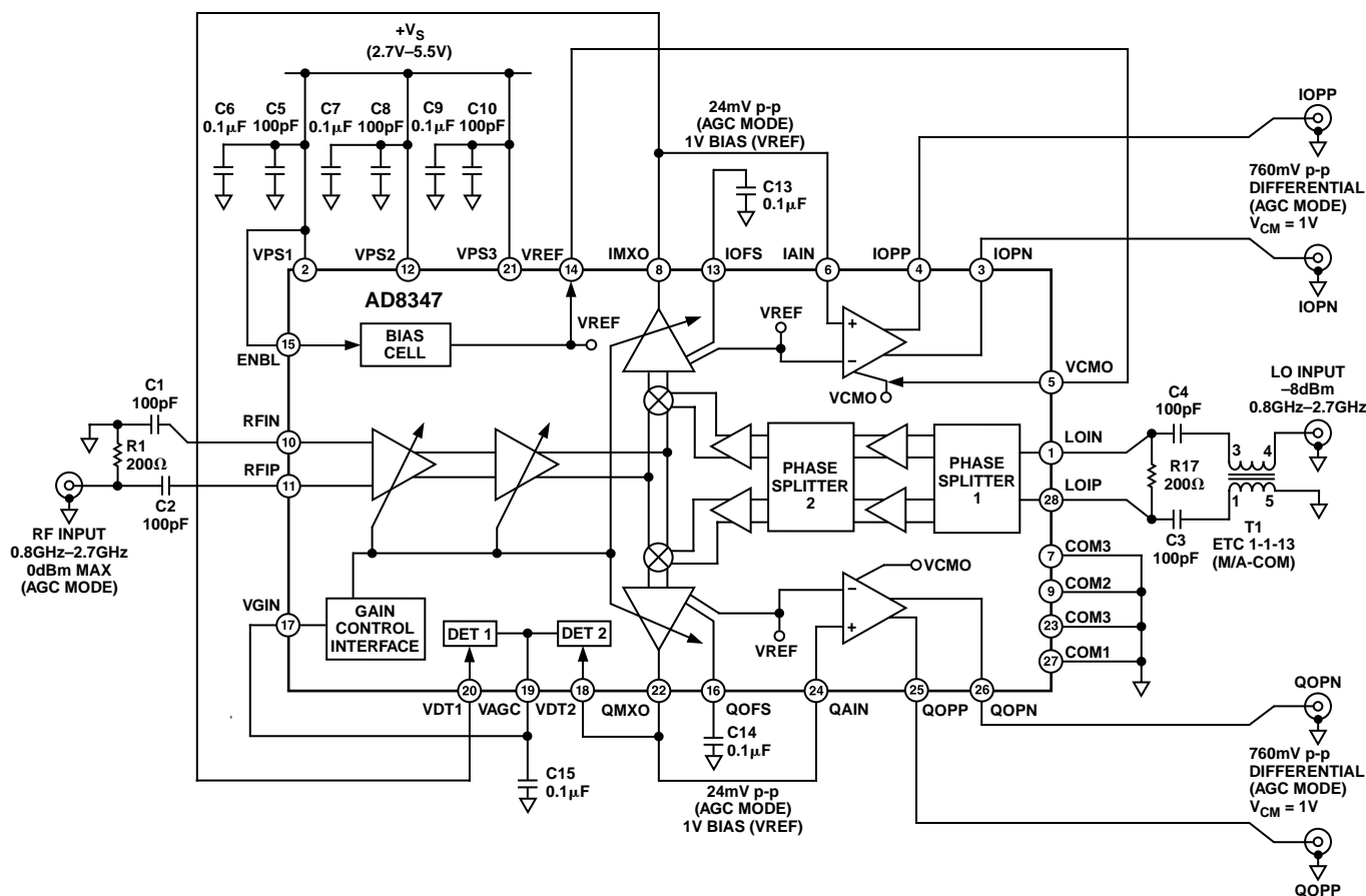
Figure 4. Basic Connections
