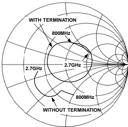
TPC 29. S_{11} of LOIN vs. F_{LO} , V_{VGIN} = 0.7\text{ V} , V_S = 5\text{ V}
