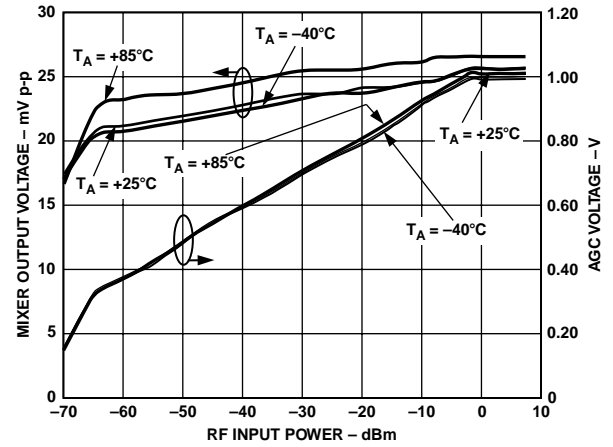
TPC 30. AGC Voltage and Mixer Output Level vs. RF Input Power, F_{LO} = 1900\text{ MHz} , F_{BB} = 1\text{ MHz} , V_S = 5\text{ V}
