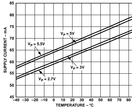
TPC 31. Supply Current vs. Temperature, V_{VGIN} = 0.7\text{ V} , V_{VCMO} = 1\text{ V}
