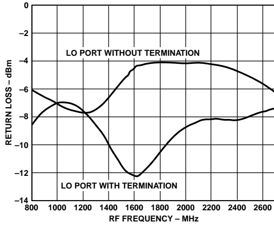
TPC 28. Return Loss of LOIP vs. F_{LO} , V_{VGIN} = 0.7\text{ V} , V_P = 5\text{ V}
