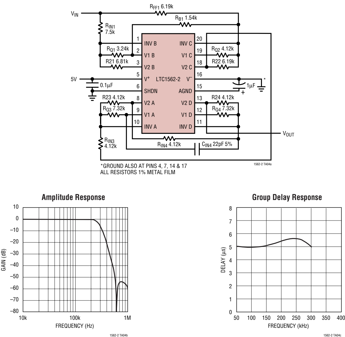
256kHz Linear Phase 6th Order Lowpass Filter with a 2nd Order Allpass Phase Equalizer, Single Supply
