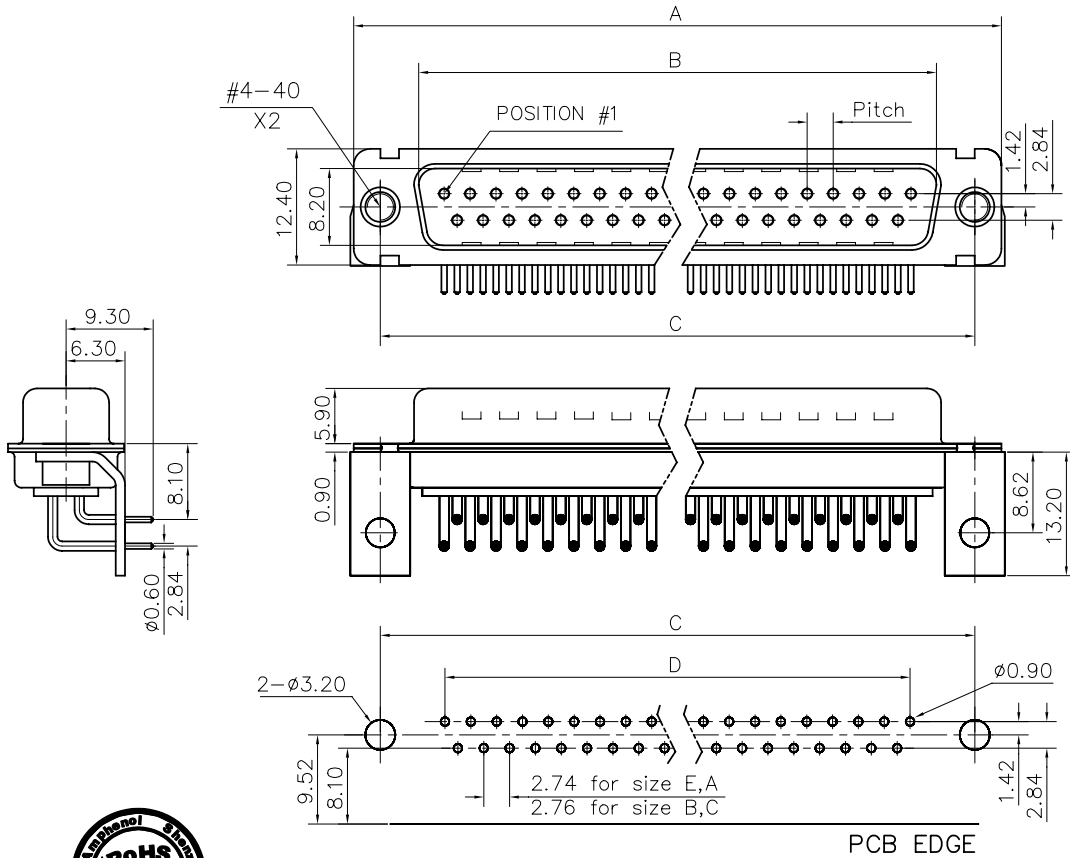
RECOMMENDED P.C.B LAYOUT (TOLERANCE +/-0.03)
