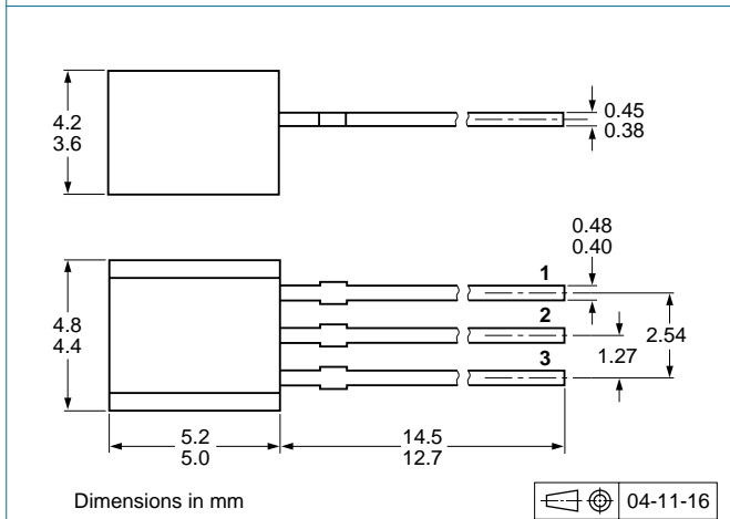
Fig 17. Package outline SOT54 (SC-43A/TO-92)
