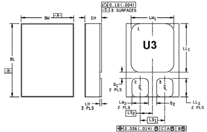
FIGURE 2 (U3) PACKAGE DIMMENSIONS
