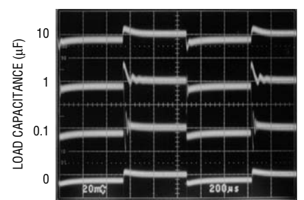
2.5V Transient Responses
