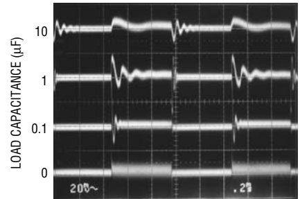
5V Transient Responses
