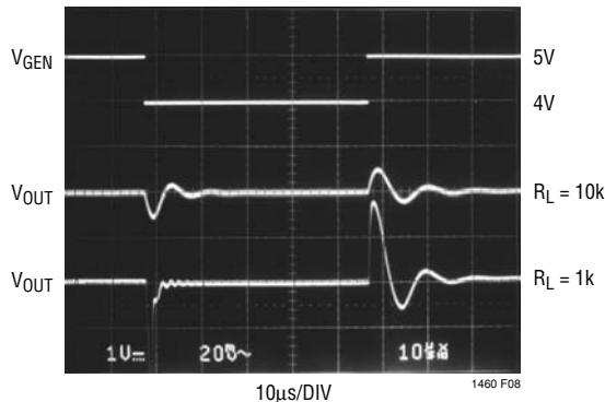
Figure 8. C_L = 0.01\mu\text{F}
