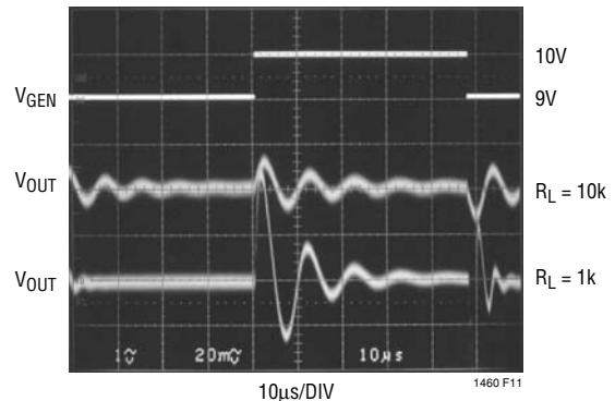
Figure 11. C_L = 0.01\mu\text{F}
