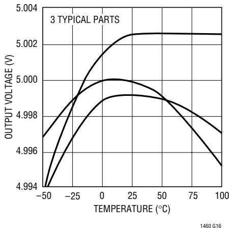
5V Output Voltage Temperature Drift
