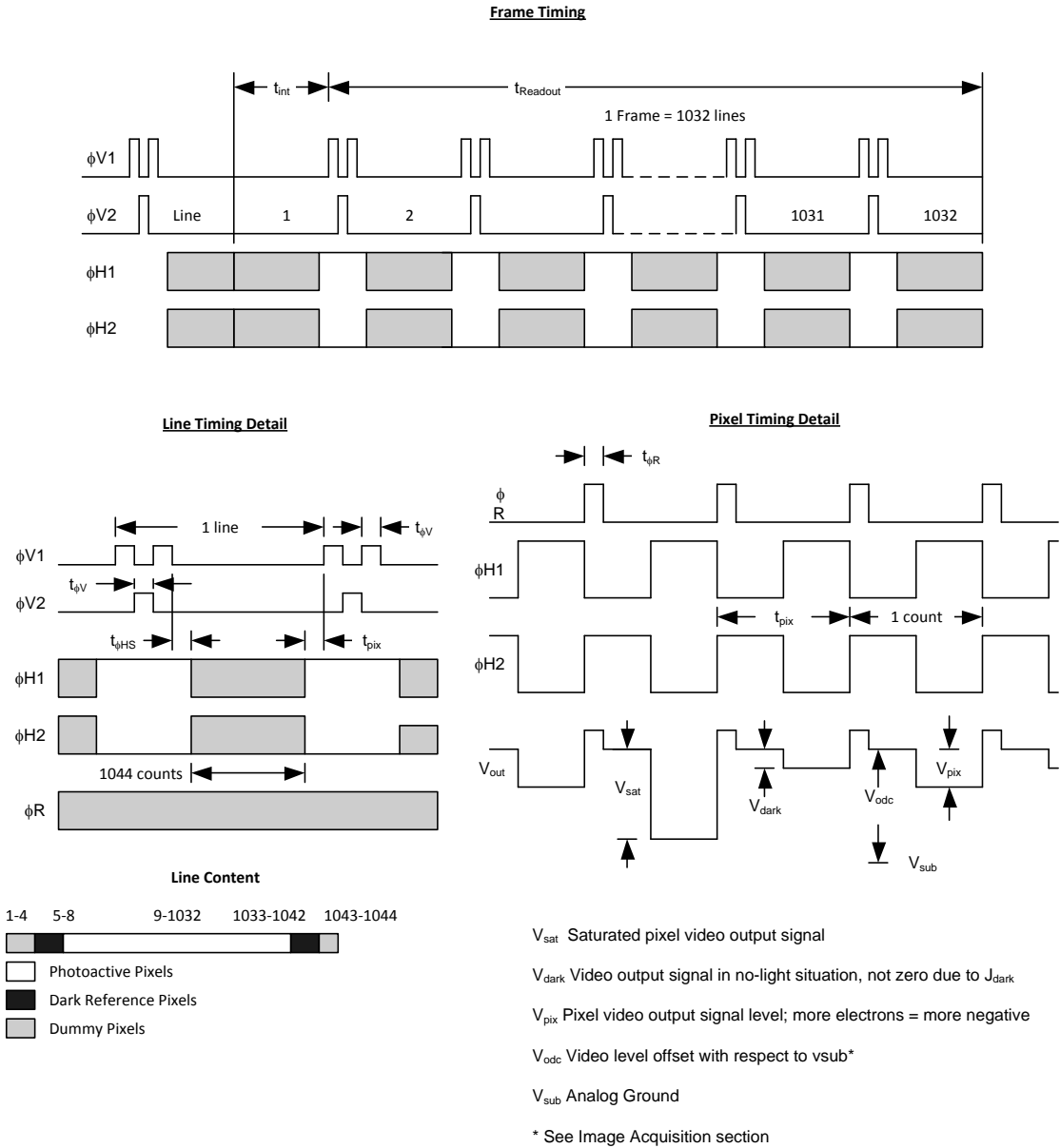
Figure 7: Timing Diagram
