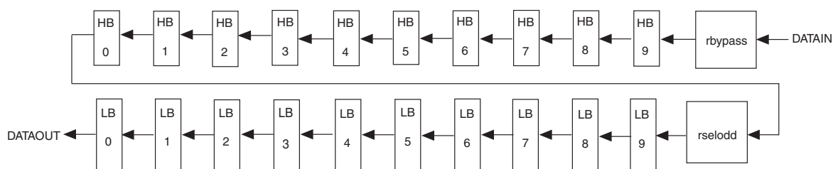
Figure 5–25. Scan Chain Bit Order
