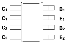
PARTMARKING DETAIL – T1049
