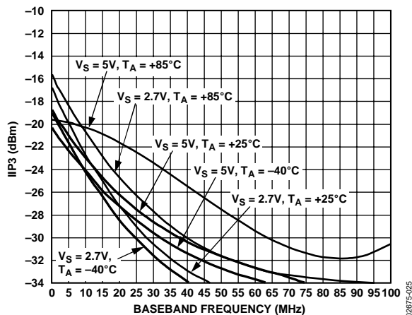
Figure 16. IIP3 vs. F_{BB} , V_{GIN} = 0.2 V, F_{LO} = 1900 MHz
