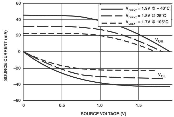
Figure 33. Driver Type C Current ( 1.8V_{DDEXT} )
