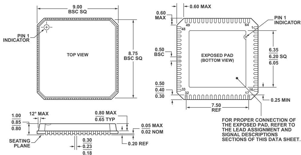
Figure 45. 64-Lead Lead Frame Chip Scale Package [LFCSP_VQ¹] Very Thin Quad (CP-64-4) Dimensions shown in millimeters
