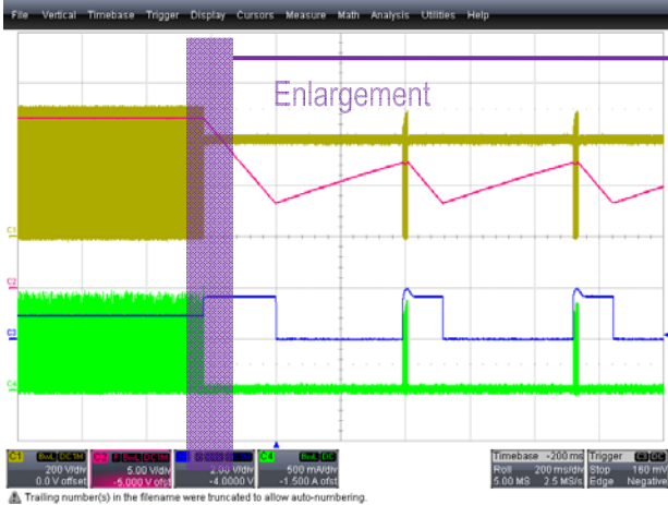
Figure 31. OSP Triggered: V_{FB} = 1.60\text{V} , 5V Output Short with 265V AC and Full-Load, CH1: V_{DS} (200V/div), CH2: V_{CC} (5V/div), CH3: V_{FB} (2V/div), CH4: I_{DS} (500mA/div), Time: 200ms/div and 10ms/div
