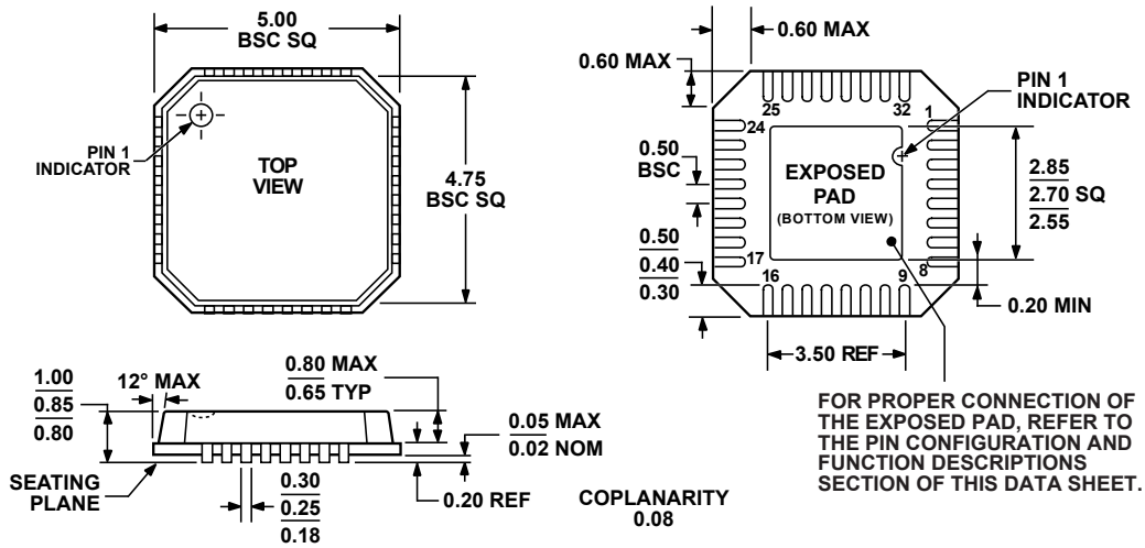
Figure 63. 32-Lead Lead Frame Chip Scale Package [LFCSP_VQ] 5 mm × 5 mm Body, Very Thin Quad (CP-32-8) Dimensions shown in millimeters
