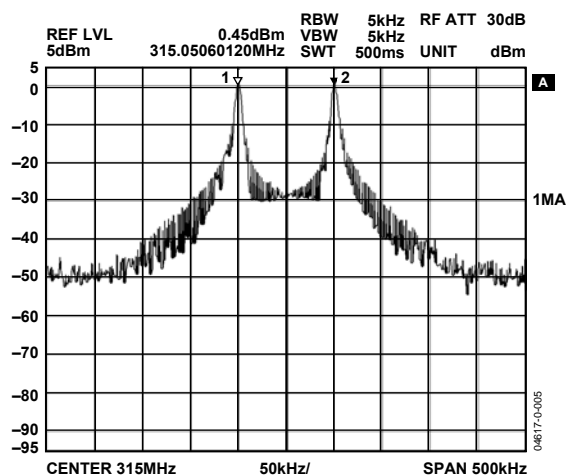
Figure 5. FSK Modulation, Power = 0 dBm, Data Rate = 1 kbps, F_{DEVIATION} = \pm 50 kHz
