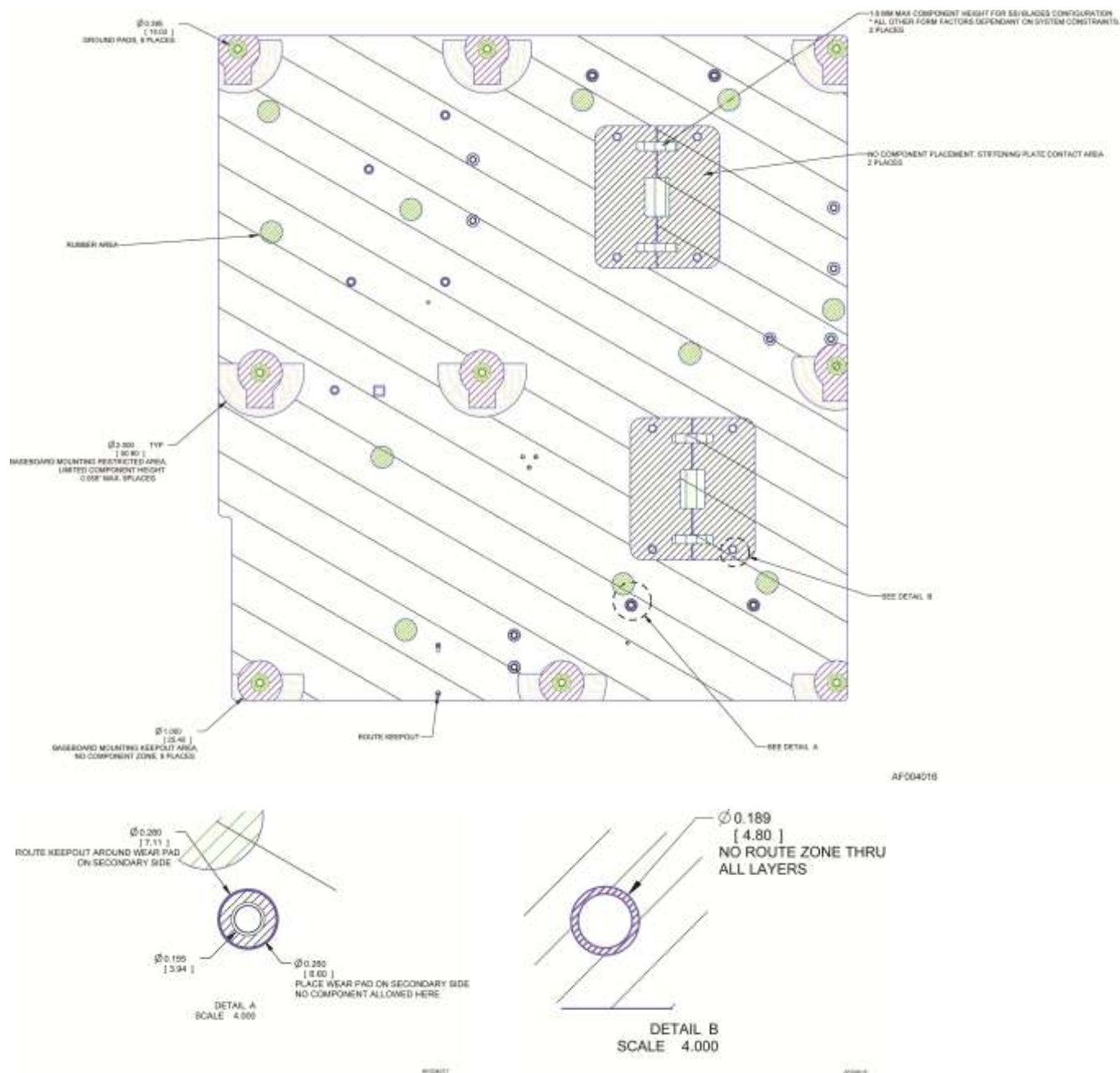
Figure 13. Second Side Keep-out Zone
