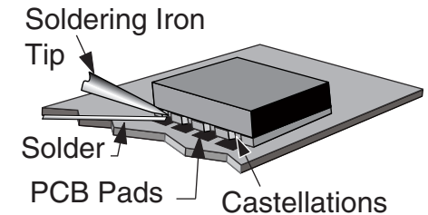
Figure 34: Soldering Technique
