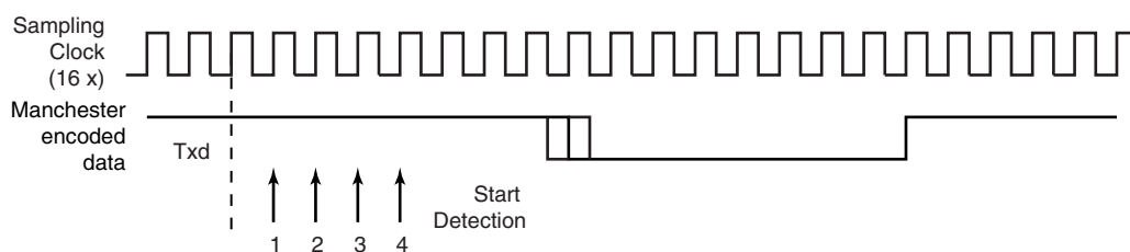
Figure 39-14. Asynchronous Start Bit Detection
