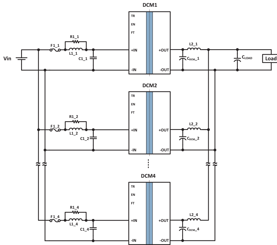
Typical Application 1: MDCM270P050M250A40 in an array of four units
