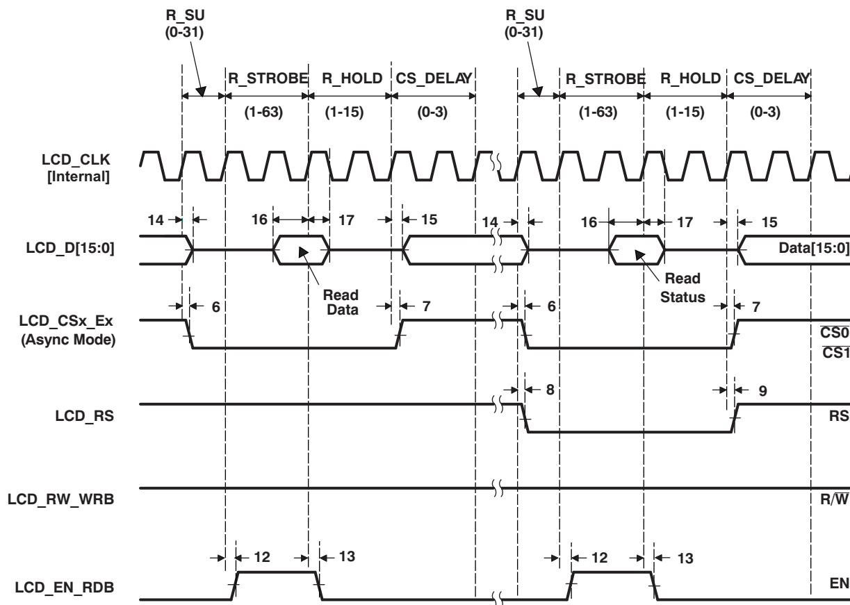
Figure 6-30. Micro-Interface Graphic Display 6800 Status
